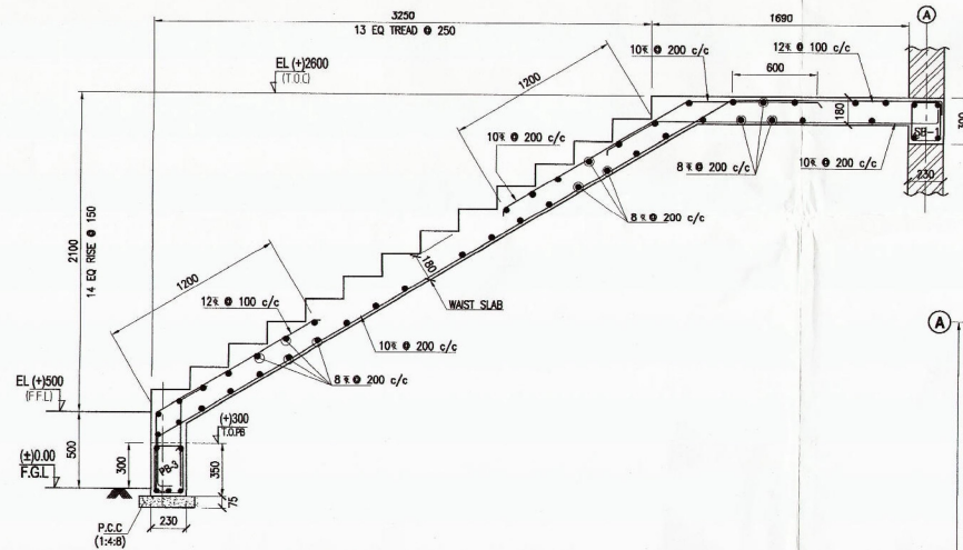
SEC 4 - 4 DET. OF STAIRCASE
