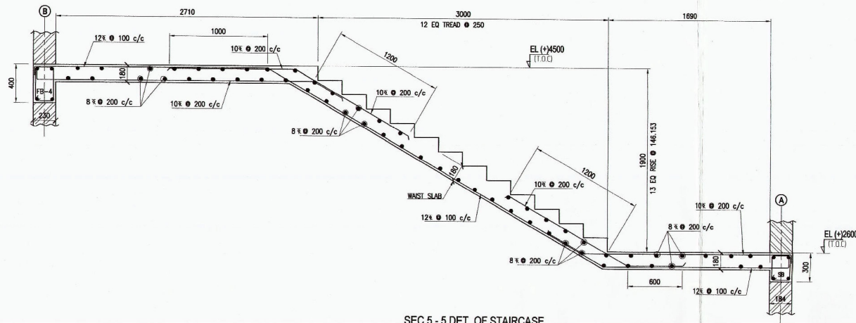
SEC 5 - 5 DET. OF STAIRCASE
