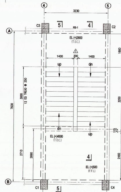
DET. LAYOUT PLAN OF STAIRCASE
